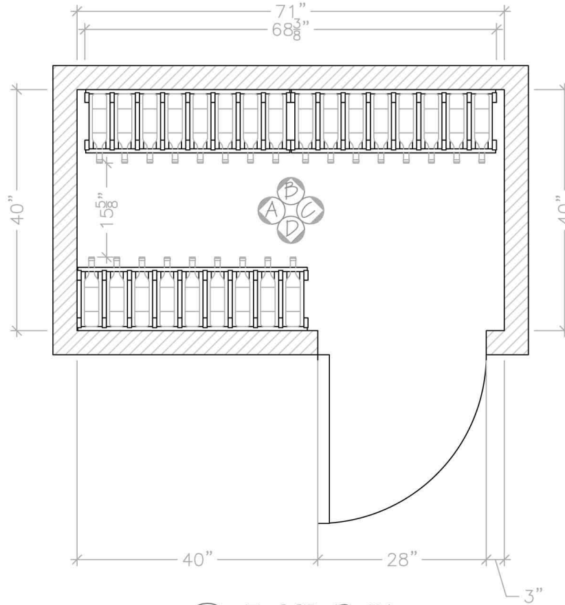
FP 1 FLOOR PLAN SCALE: TO FIT
